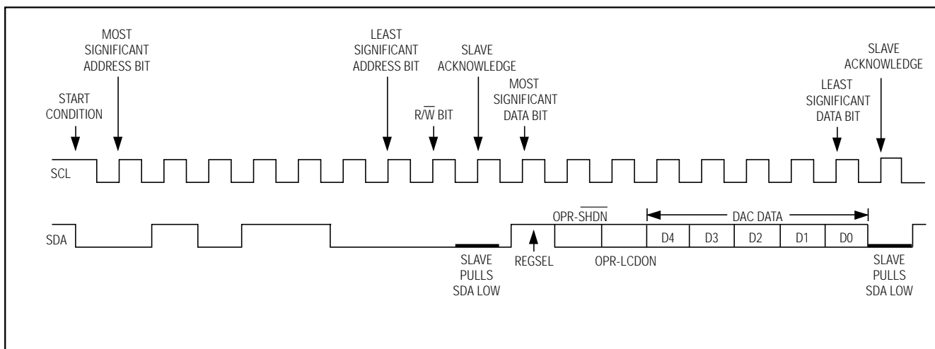
Figure 8. MAX1621 Serial-Interface Single-Byte Write Example (REGSEL = 1)
