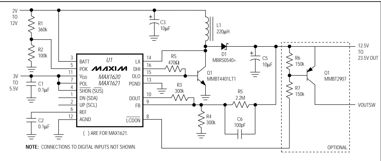
Figure 10. Positive Output with Bipolar Switching Transistor
