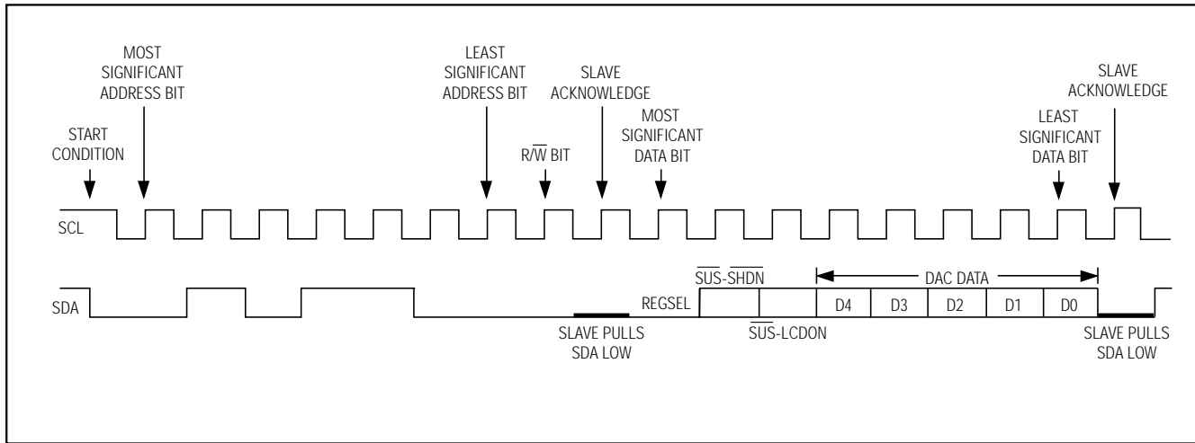
Figure 7. MAX1621 Serial-Interface Single-Byte Write Example (REGSEL = 0)
