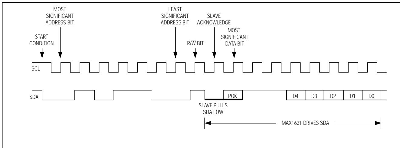
Figure 9. MAX1621 Serial-Interface Read Example
