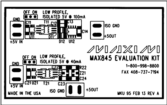
Figure 2. MAX845 EV Kit Component Placement Guide—Component Side
