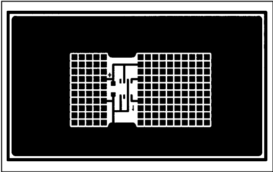
Figure 4. MAX845 EV Kit PC Board Layout—Solder Side
