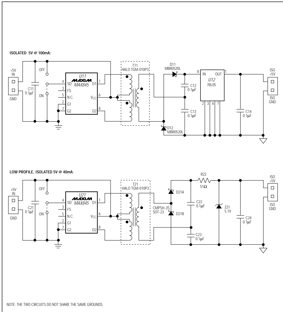
Figure 1. MAX845 EV Kit Schematic
