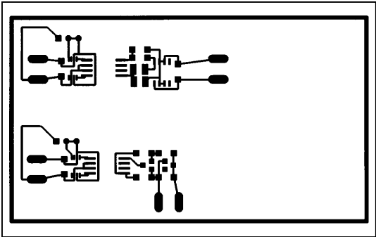
Figure 3. MAX845 EV Kit PC Board Layout—Component Side
