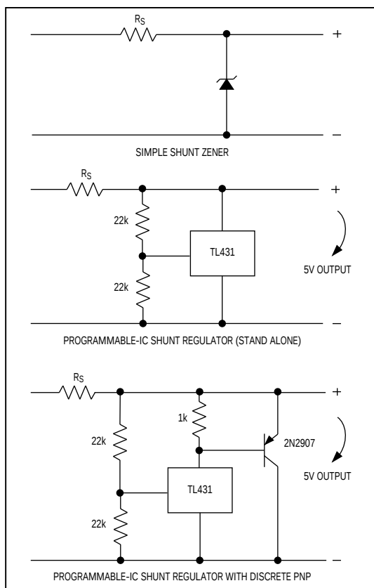
Figure 12. Shunt-Regulator Circuits
