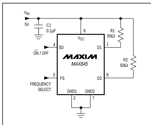
Figure 1. Test Circuit
