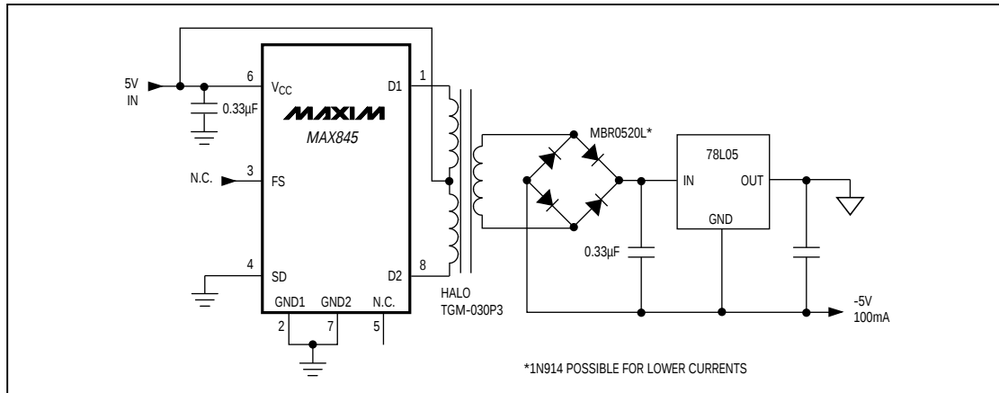
Figure 5. Low-Noise Supply
