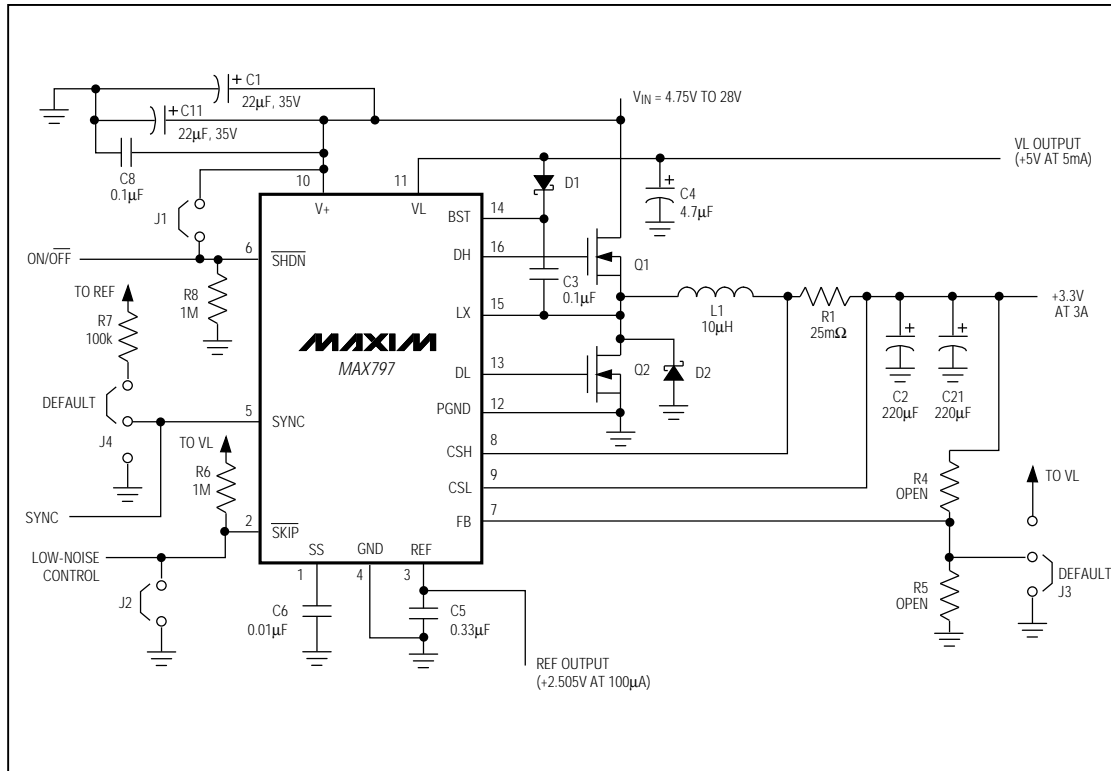
Figure 1. MAX797 EV Kit Schematic
