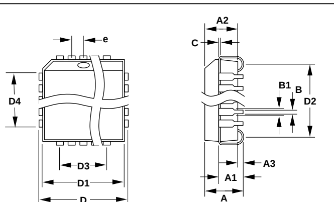
Q PACKAGE PLASTIC LEADED CHIP CARRIER
