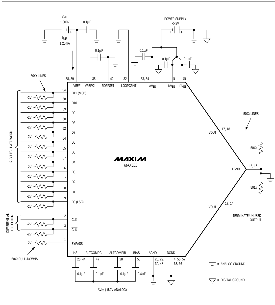
Figure 4. Typical Application
