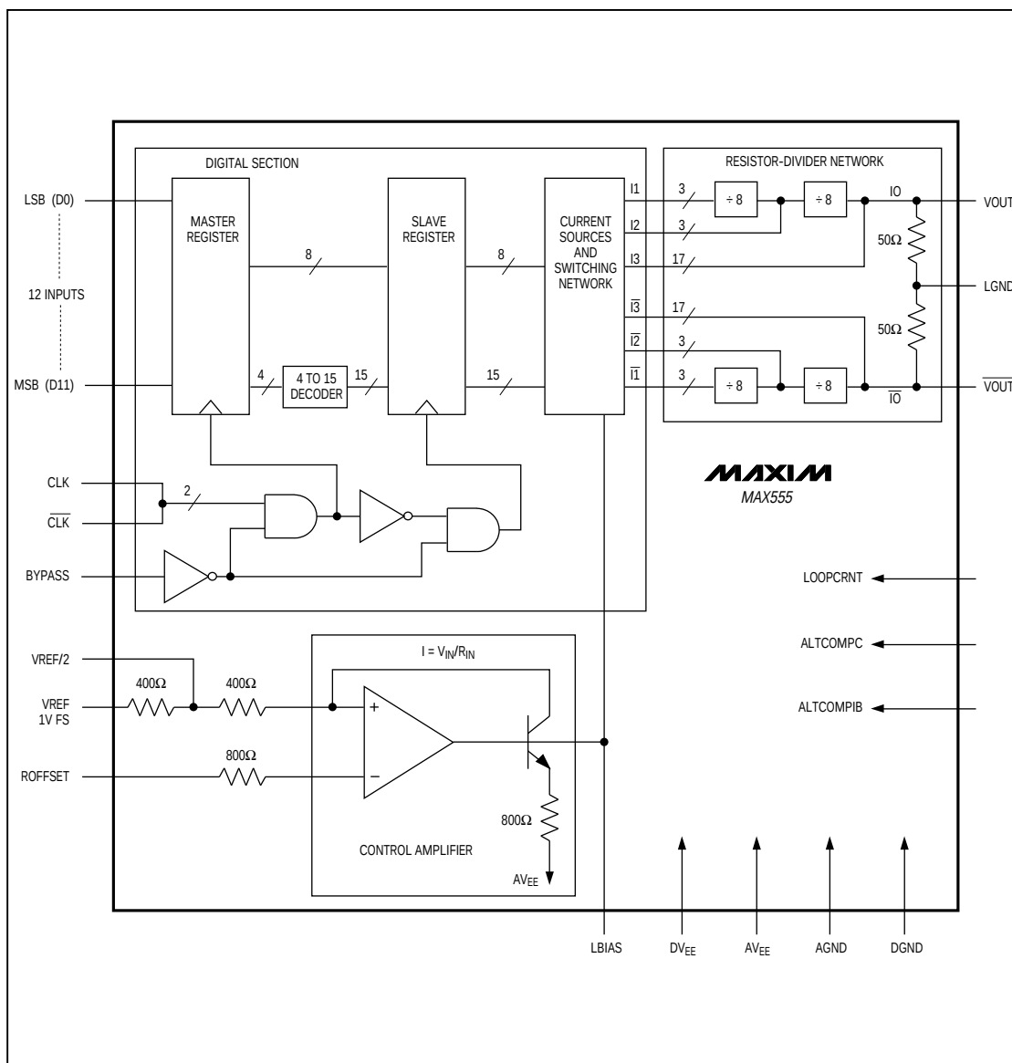
Figure 1. Functional Diagram
