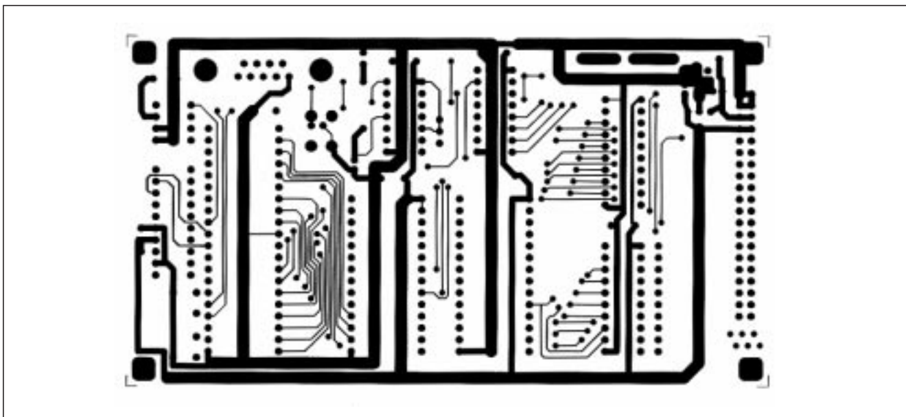
Figure 3. 80C32 Module Component-Side Layout (x1)
