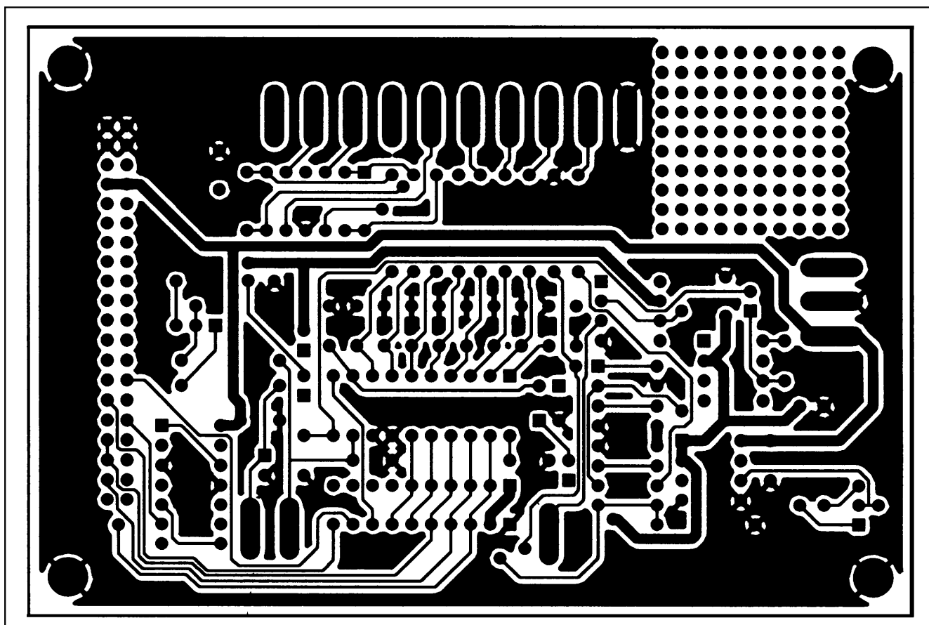
Figure 4. MAX147EV Kit PC Board Layout—Solder Side
