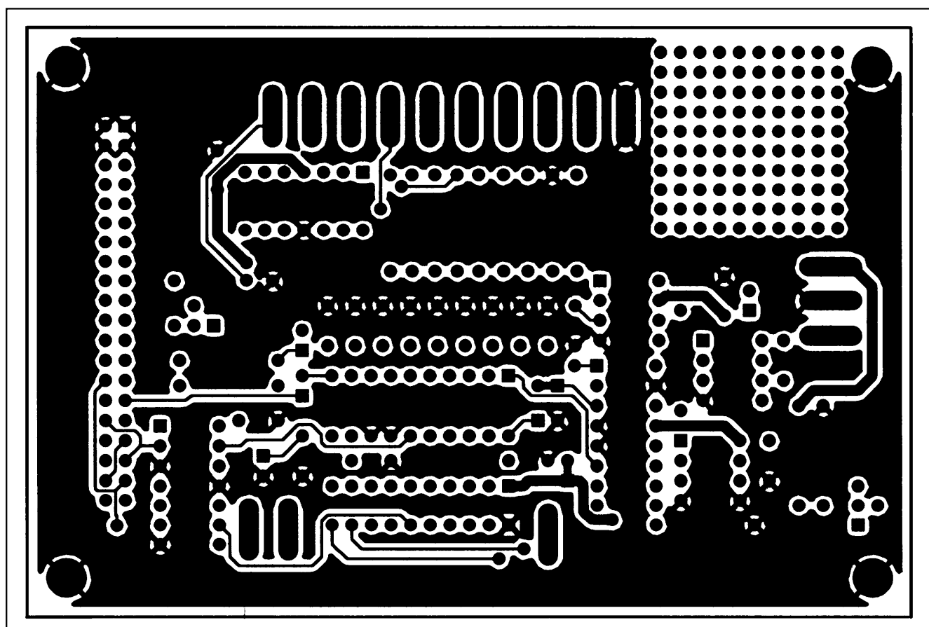
Figure 3. MAX147EV Kit PC Board Layout—Component Side
