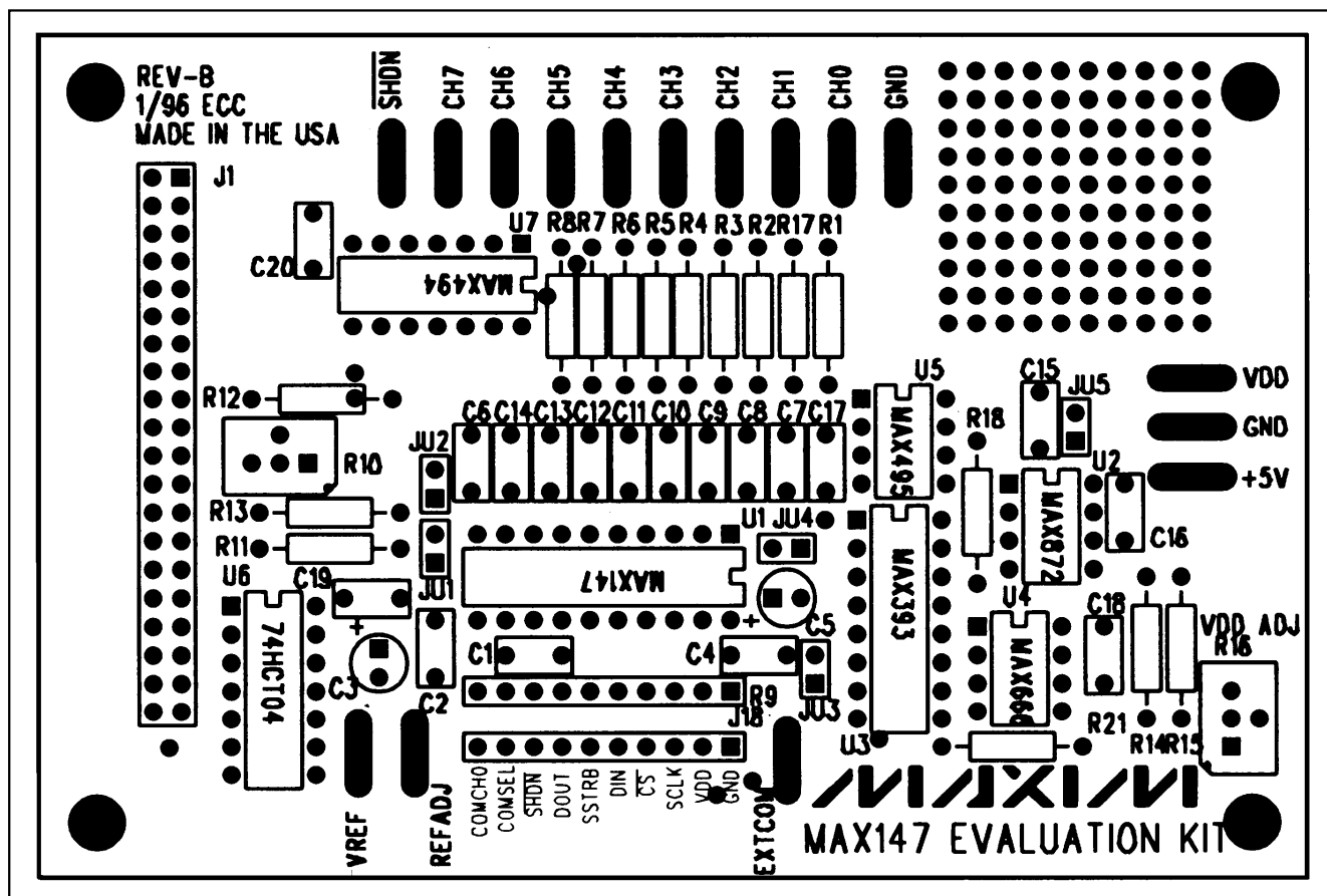
Figure 2. MAX147EV Kit Component Placement Guide—Component Side
