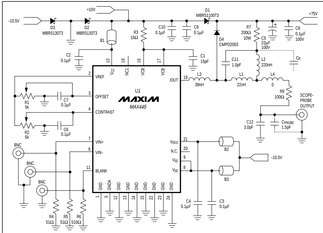
Figure 1. MAX445 EV Kit Schematic Diagram
