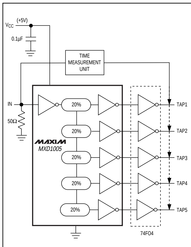
Figure 2. Test Circuit
