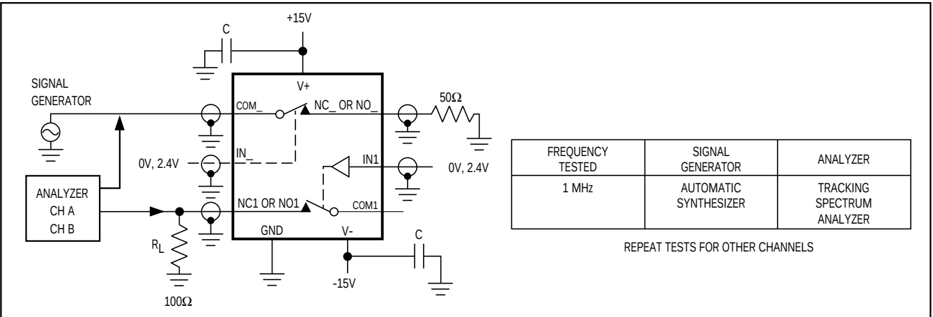
Figure 8. Crosstalk
