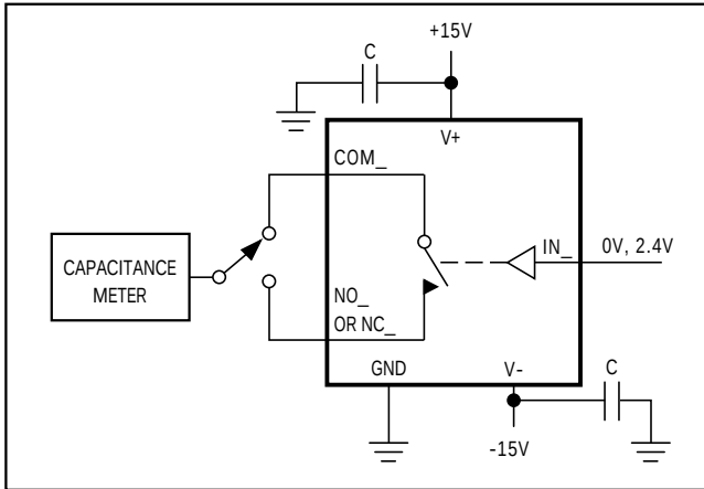
Figure 3. Channel-Off Capacitance
