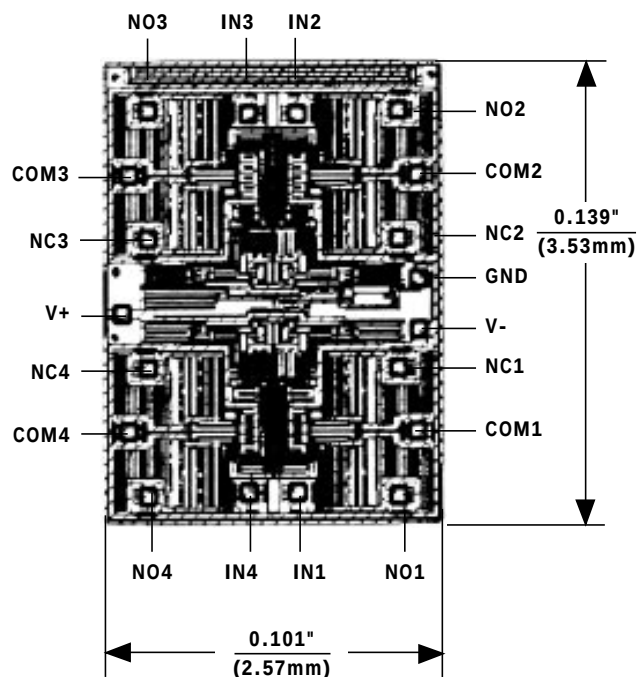
Chip Topography
