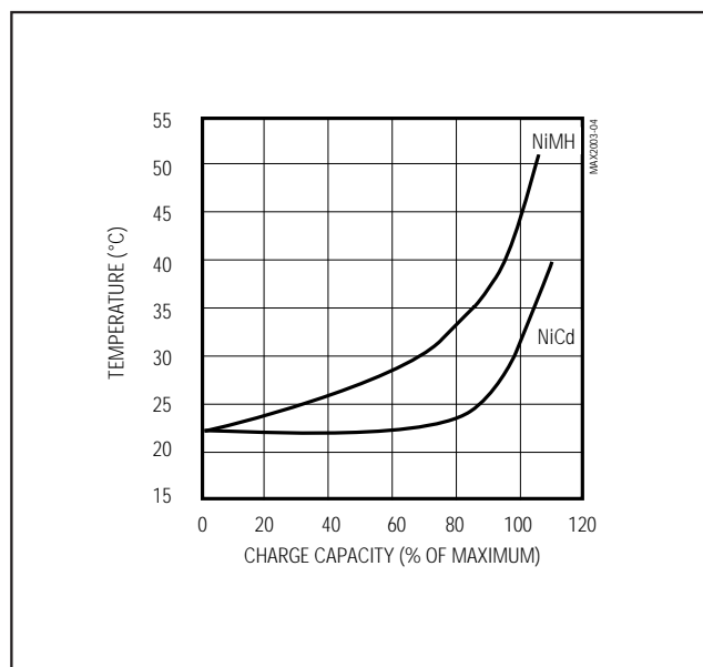
Figure 4. Temperature-Charge Characteristics of NiCd and NiMH Batteries
