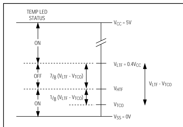
Figure 5. Temperature Measurement Scale
