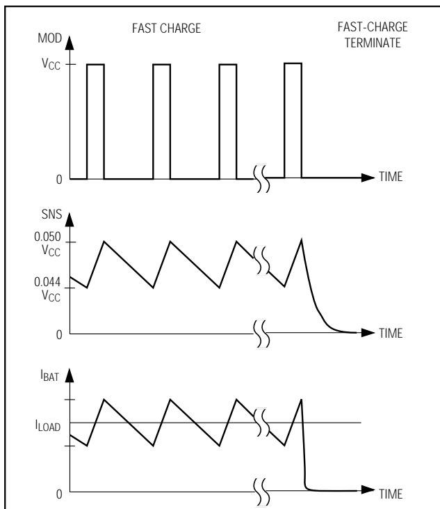
Figure 7. Current Regulation with an SNS Resistor
