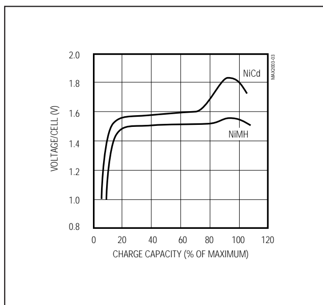
Figure 3. Voltage-Charge Characteristics of NiCd and NiMH Batteries
