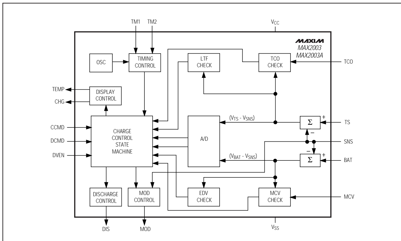
Figure 2. Block Diagram
