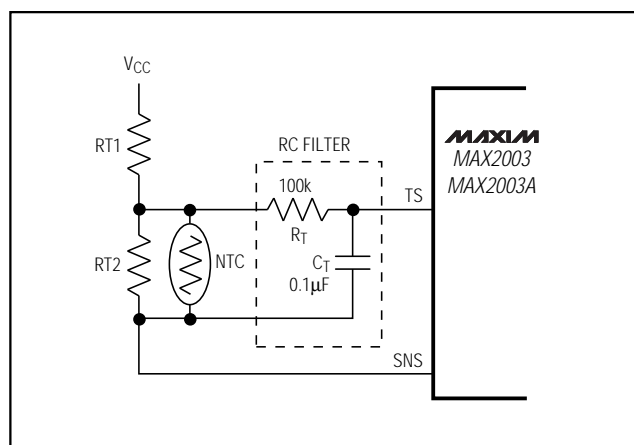
Figure 6. Thermistor Configuration for Temperature Measurement
