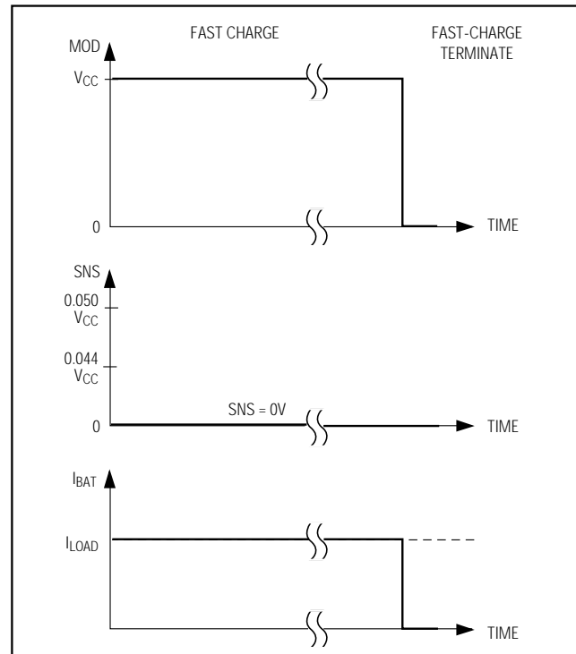
Figure 8. Current Regulation without an SNS Resistor
