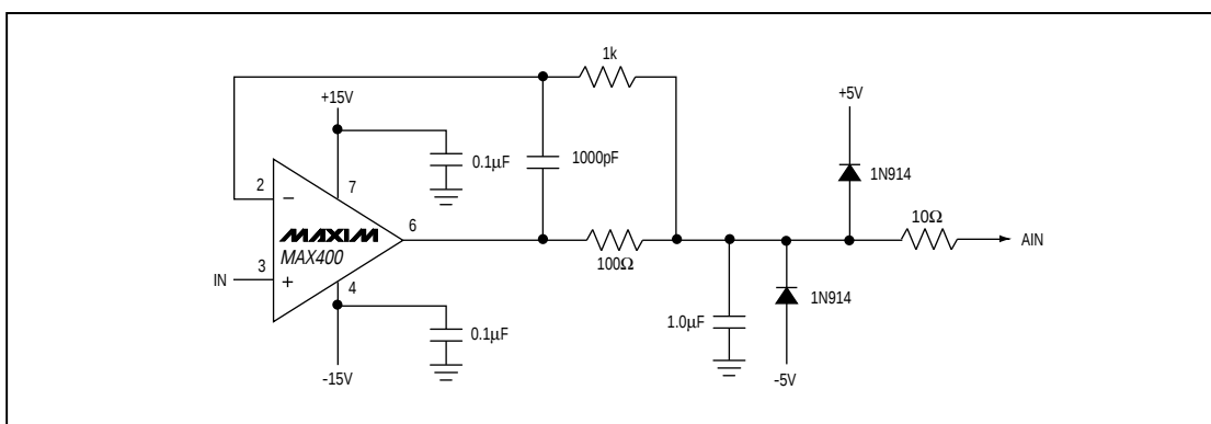
Figure 14. MAX400 Drives AIN for Low-Frequency Use
