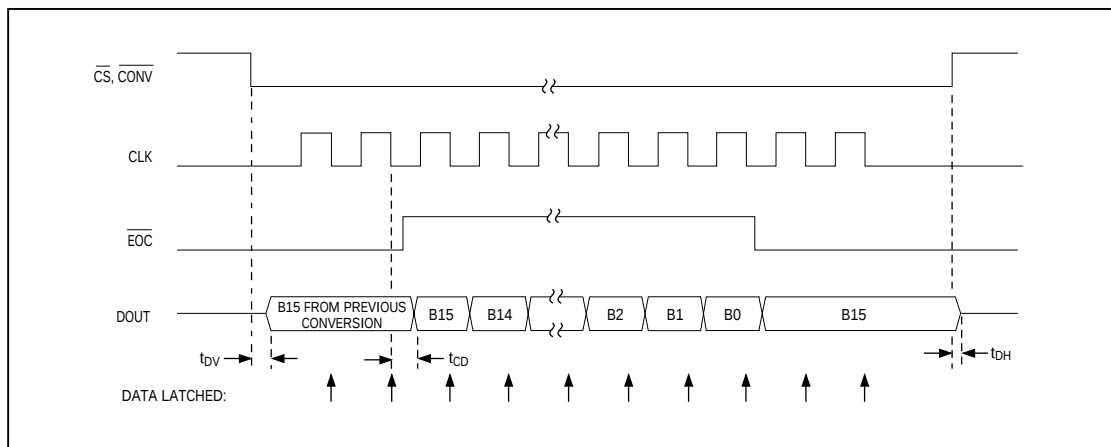
Figure 18. Timing Diagram for Circuit of Figure 17 (Mode 1)
