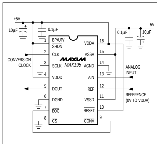
Figure 8. MAX195 in the Simplest Operating Configuration
