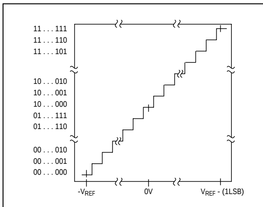
Figure 30. MAX195 Bipolar Transfer Function
