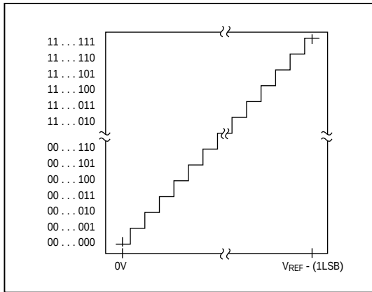
Figure 29. MAX195 Unipolar Transfer Function
