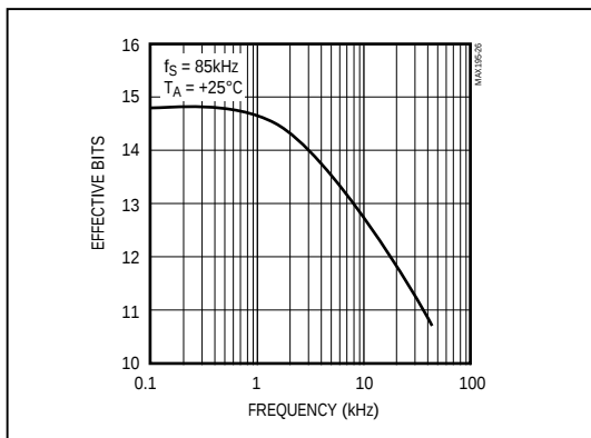
Figure 26. Effective Bits vs. Input Frequency
