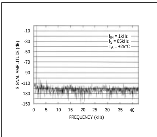
Figure 25. MAX195 FFT Plot
