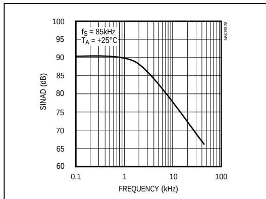
Figure 28. Signal-to-Noise + Distortion vs. Frequency
