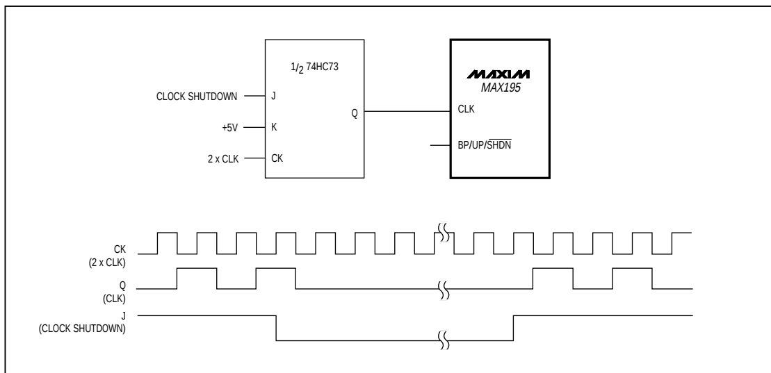
Figure 24. Circuit to Stop Free-Running Asynchronous CLK
