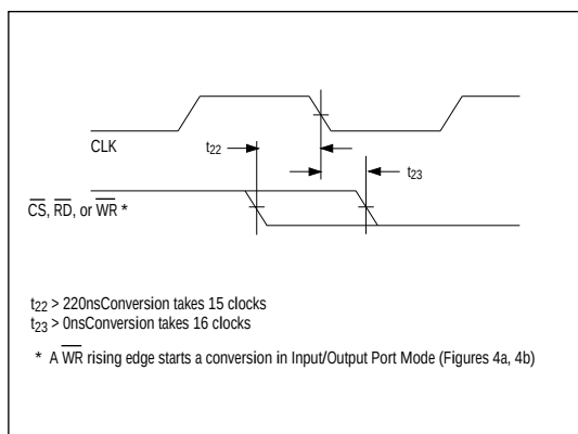
Figure 8. \overline{\text{CS}} , \overline{\text{RD}} , or \overline{\text{WR}} to CLK Setup and Hold Time for Synchronous Operation
