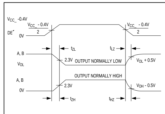
Figure 8. Driver Enable and Disable Times
