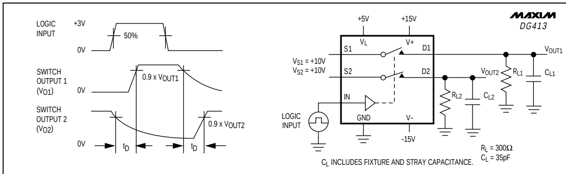
Figure 3. DG413 Break-Before-Make
