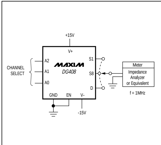
Figure 8. Source/Drain Capacitance
