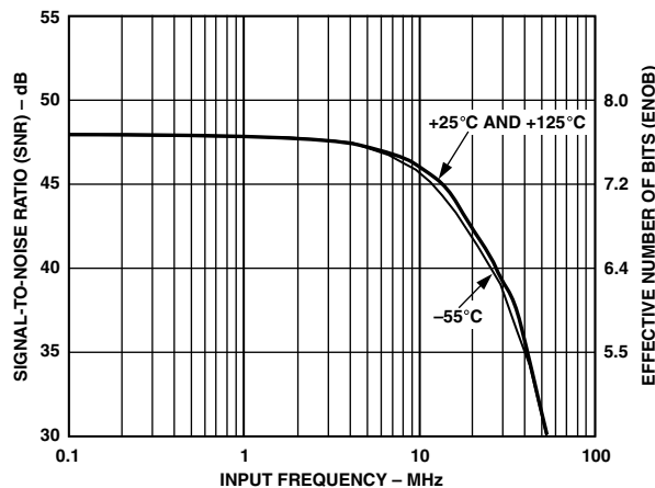
Figure 7. AD9058 Dynamic Performance vs. Analog Input Frequency
