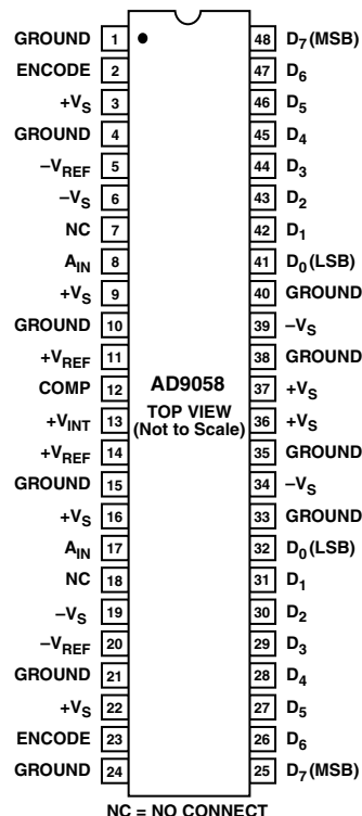
AD9058AJD/AKD Pinouts
