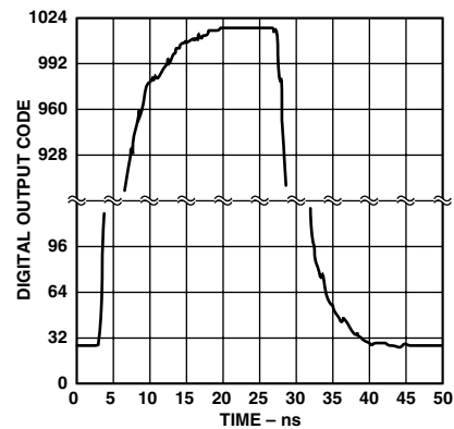
TPC 6. Transient Response (Expanded View)
