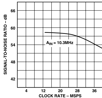
TPC 3. SNR vs. Clock Rate
