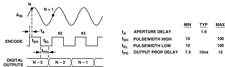
Figure 1. Timing Diagram
