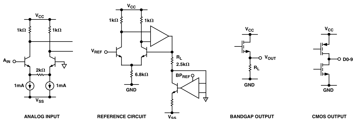
Figure 2. Equivalent Circuits
