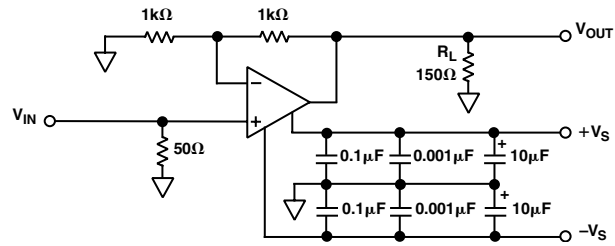
TPC 18. Test Circuit; Gain = +2
