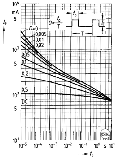
Figure 16. Permissible pulse load D =parameter, T_A=25^\circ\text{C} , I_F=f(t_D)
