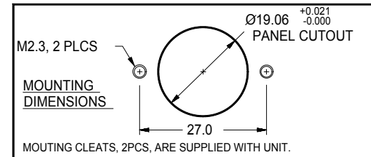
FIGURE 1 OUTLINE DIMENSIONS
