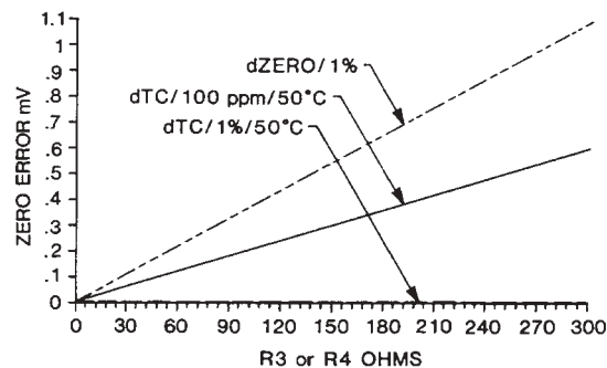
Figure 10. R 3 or R 4 Resistor Tolerance
