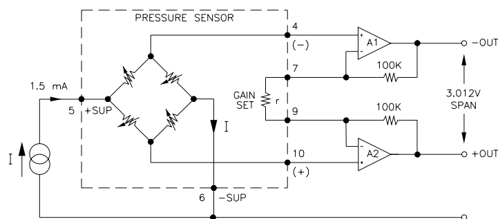
FIGURE 1: BOTTOM ENTRY FOR GAGE
