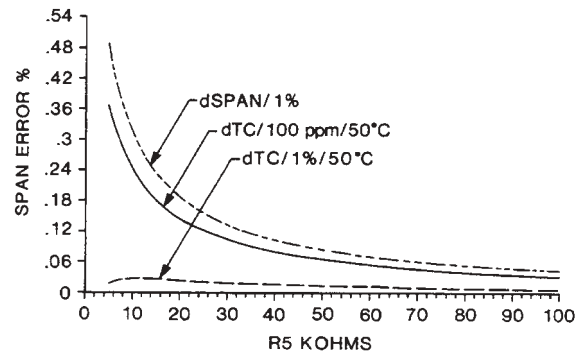
Figure 11. R 5 Resistor Tolerance
