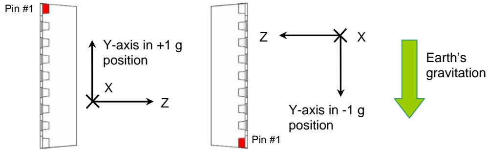
Figure 21. SCA3000 positions for Y-axis sensitivity measurement.
