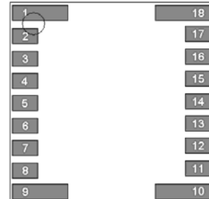
Figure 14. SCA3000 pin numbers.
