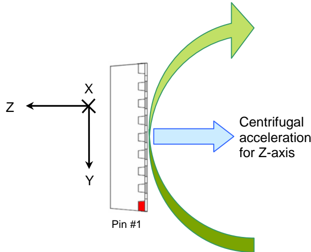
Figure 22. Centrifugal acceleration applied for SCA3000 Z-axis.
