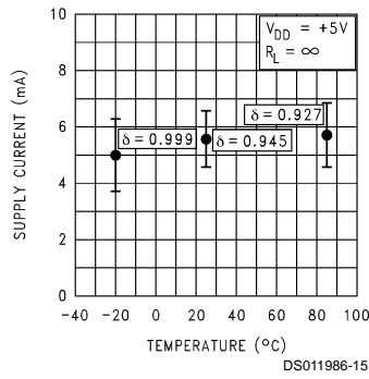
Supply Current Distribution vs Temperature
