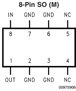
Top View Order Number LM2936M-5.0, LM2936HVMA-5.0 See NS Package Number M08A
