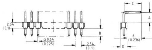
Single Row-Right Angle Pins
