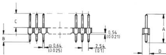
Single Row-Straight Pins
