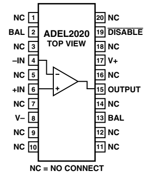
20-Lead SOIC (R)
