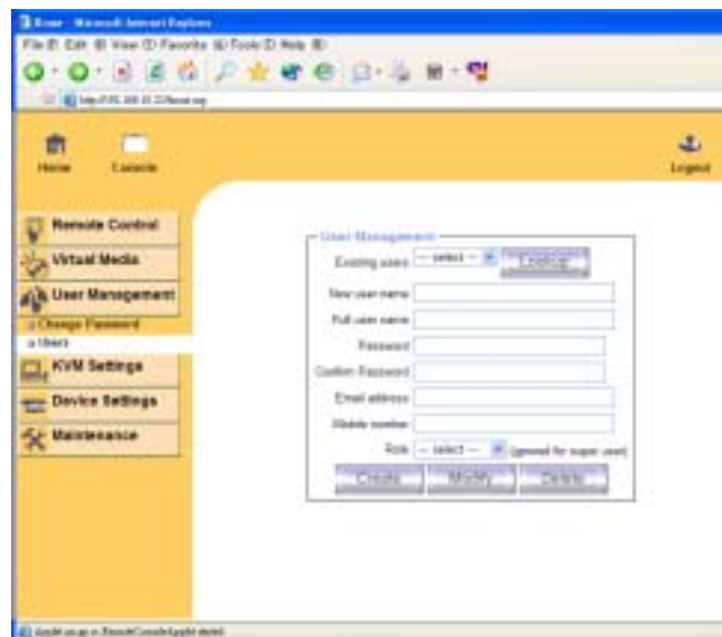
Figure 6-13. Set User
