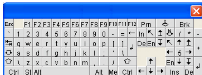
Figure 5-12. Soft Keyboard
