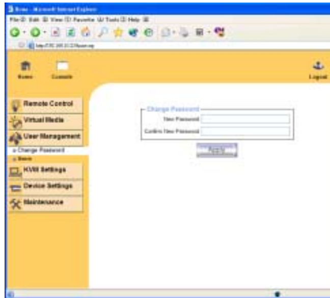
Figure 6-12. Set password
