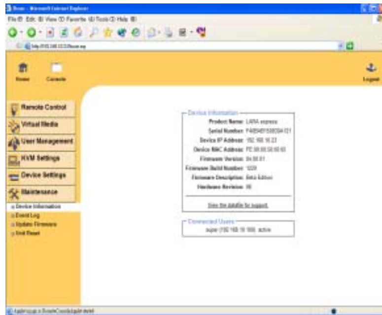
Figure 6-31. Device Information
