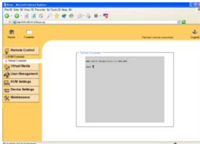
Figure 6-2. Telnet Console
