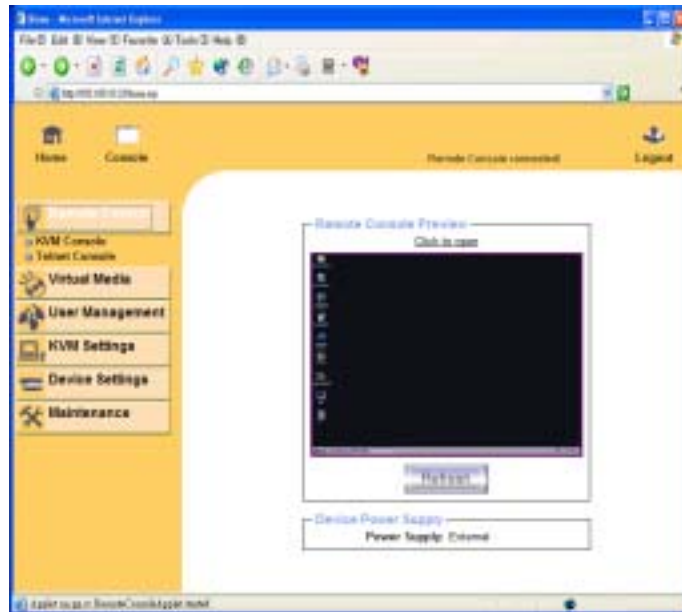
Figure 6-1. KVM Console
