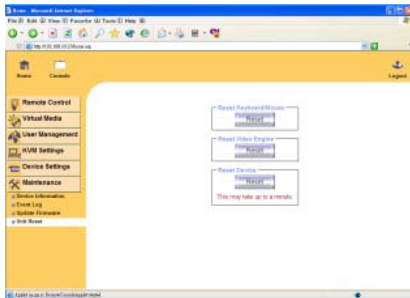
Figure 6-35 Unit Reset
