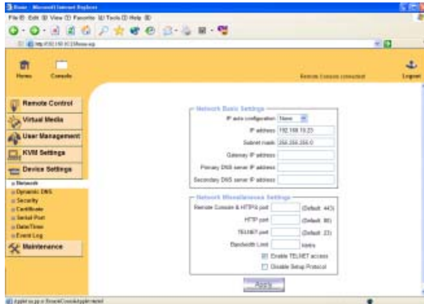
Figure 6-19. Network Settings
