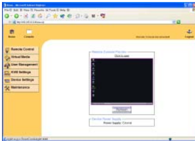
Figure 5-3. Main page
