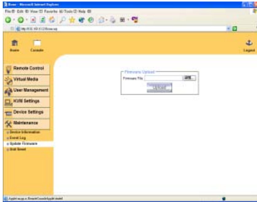
Figure 6-34. Update Firmware
