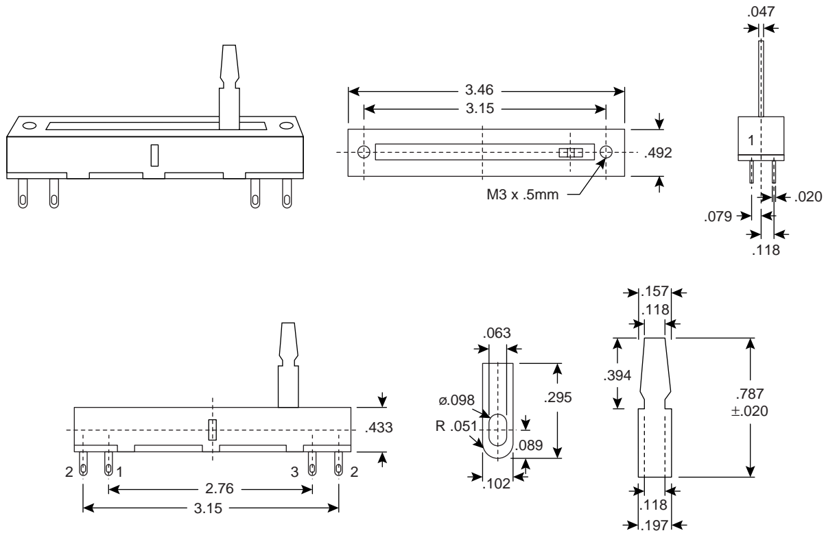
Dimensions (In.)
