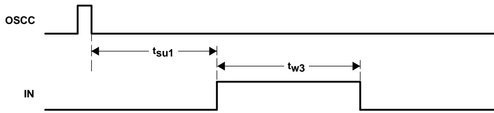
Figure 3-2. VTR Generation
