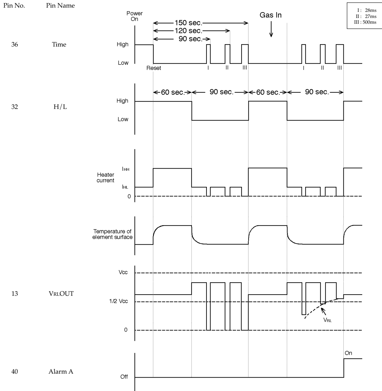
Fig. 5 - Timing chart
