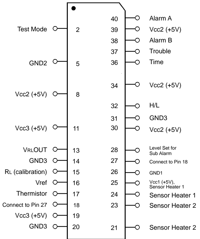
Fig. 2 - Pin connection of IC Unit (top view)
