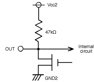
Fig. 7c - Pins 32, 36
