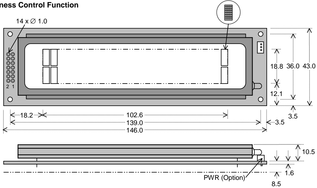
Dimensions in mm & subject to tolerances. Mounting holes 2.5mm dia.
